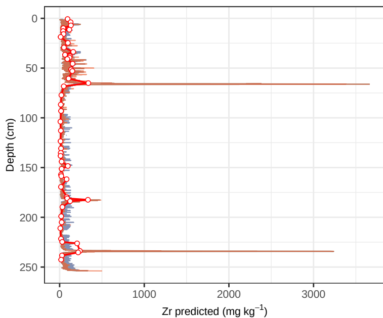
Site KER1 – Zr (depth, multivariate)
